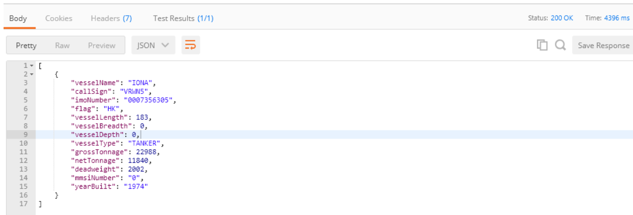
Figure 2-2: API (JSON) Response as shown on Postman
